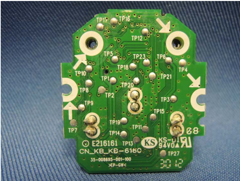
Door Bell Camera Board PCB rear side
