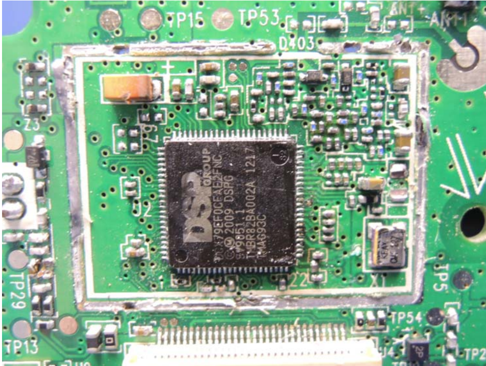
Door Bell Oscillator PCB comp side
