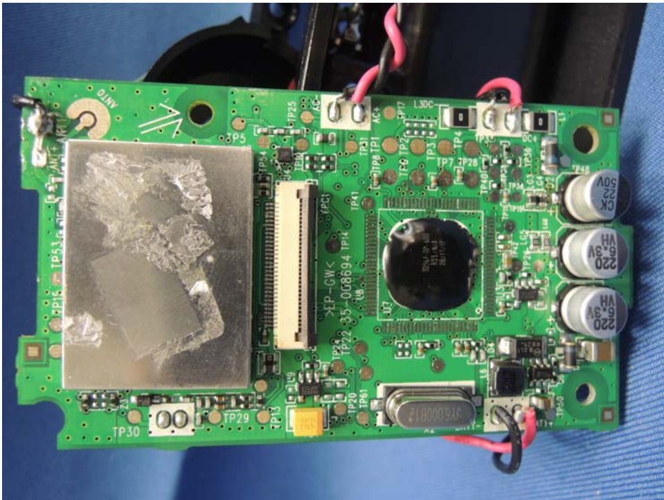
Door Bell Main PCB comp side
