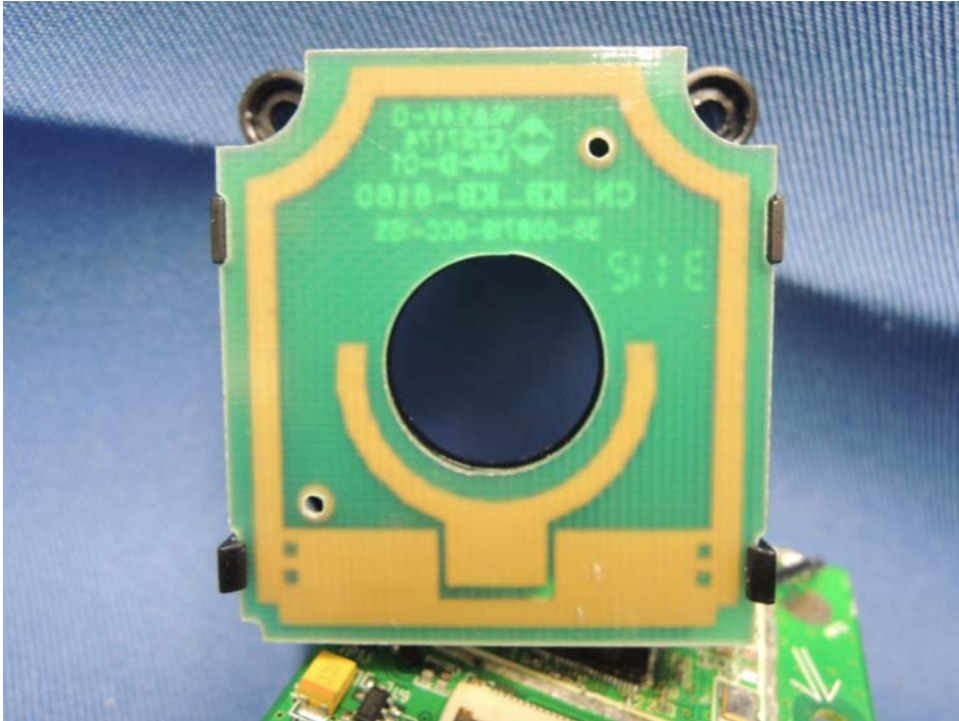
Door Bell Antenna PCB rear side
