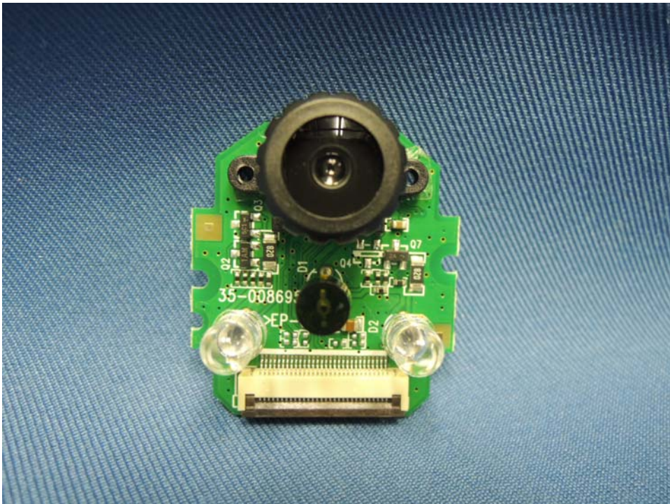
Door Bell Camera Board PCB front side (View 1)
