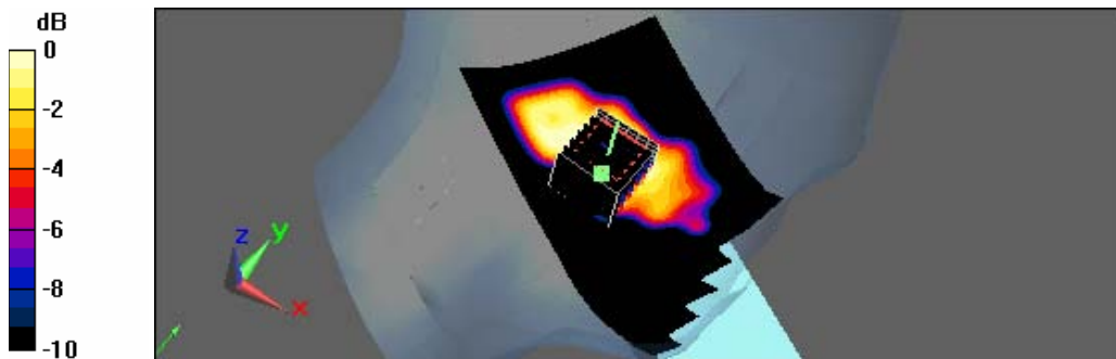
0 dB = 0.00441mW/g
