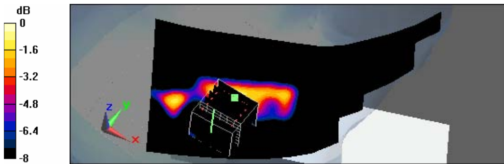
0 dB = 0.00808mW/g
