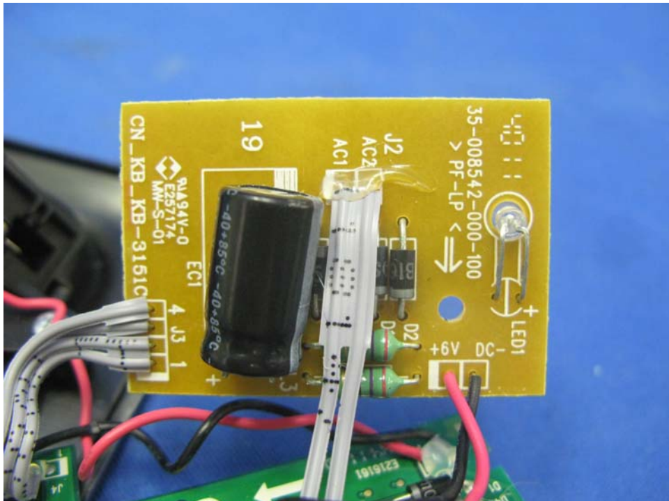
Base Unit LED front side (View 1)
