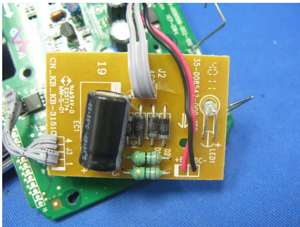
Base Unit LED front side (View 2)
