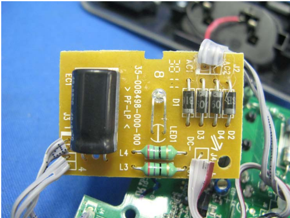
Base Unit Page Key and LED rear side
