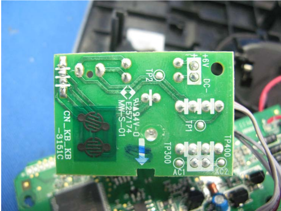
Base Unit Page Key and LED front side
