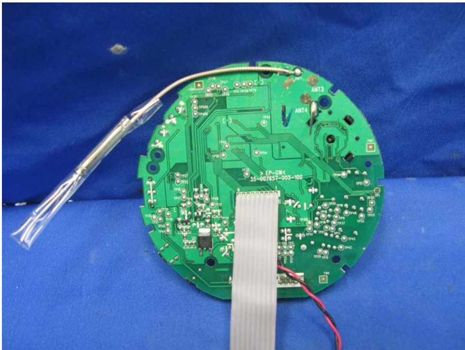
Base Unit PCB Antenna 1
