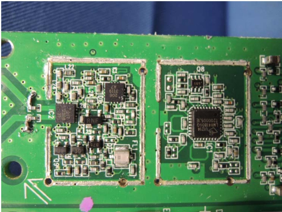
Deskset Unit Oscillator PCB comp side
