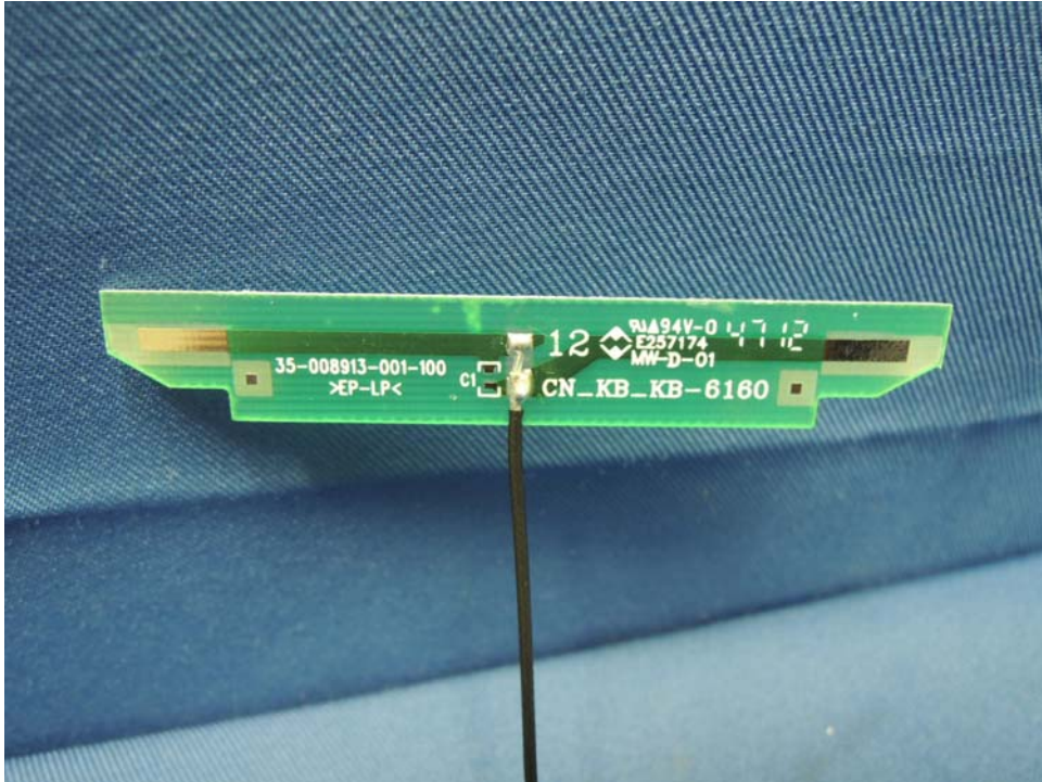
Deskset Antenna 1 rear side
