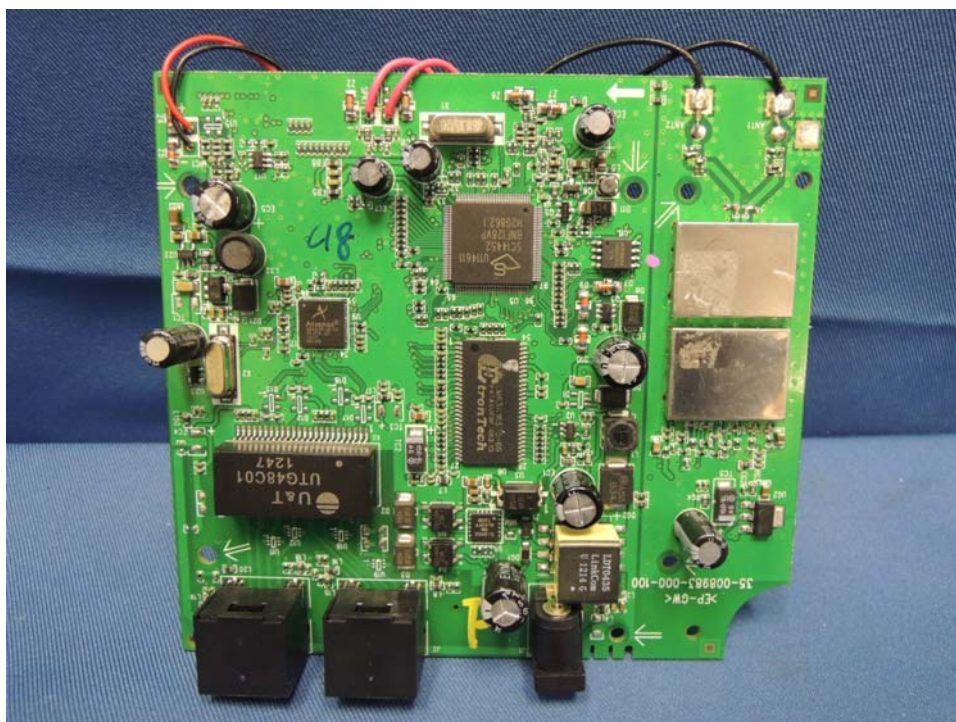
Deskset Unit Main PCB comp side
