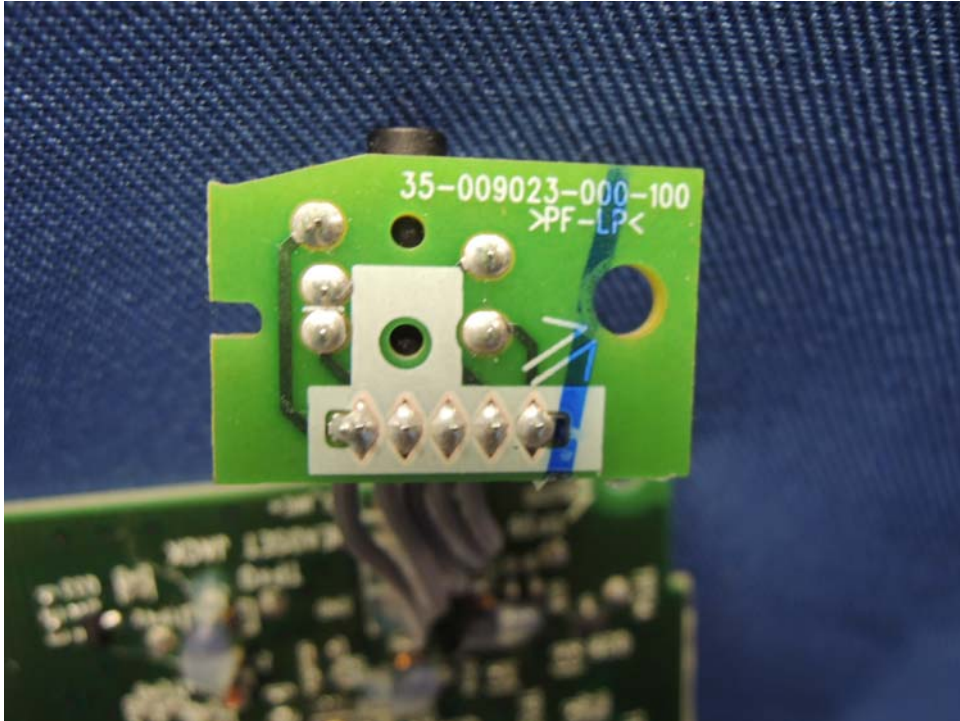
Deskset Headset PCB Board rear side
