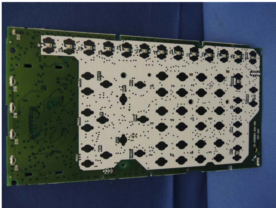
Deskset Keypad front side (View 2)
