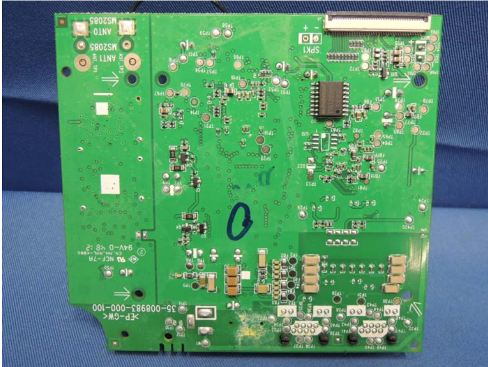
Deskset Unit Main PCB solder side
