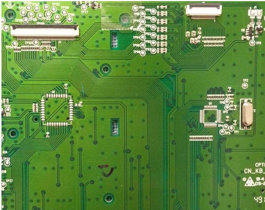
Deskset Keypad and Display rear side (View 2)
