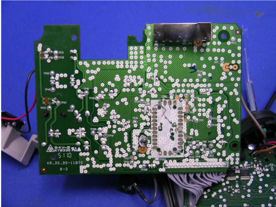
Base Unit Main PCB solder side (View 3)
