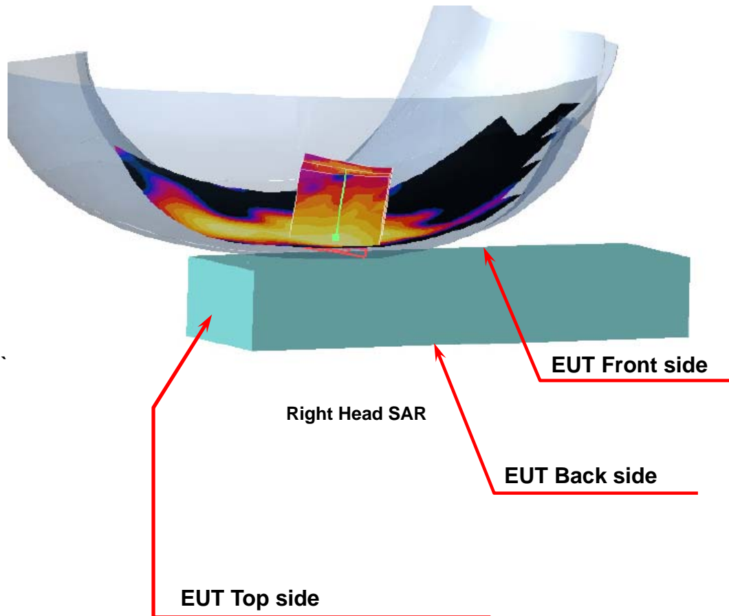
Figure 2. Right Head SAR Test Setup (Cheek)
