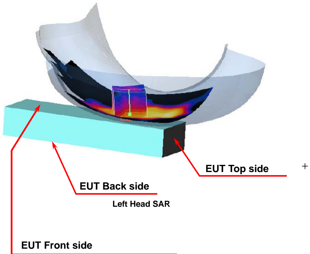
Figure 4. Left Head SAR Test Setup (Cheek)
