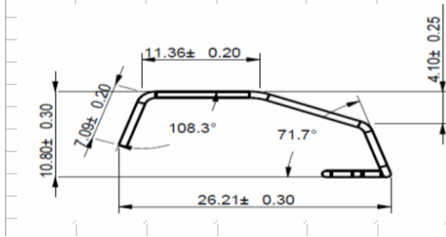
DM221 PU Antenna Physical Dimensions
