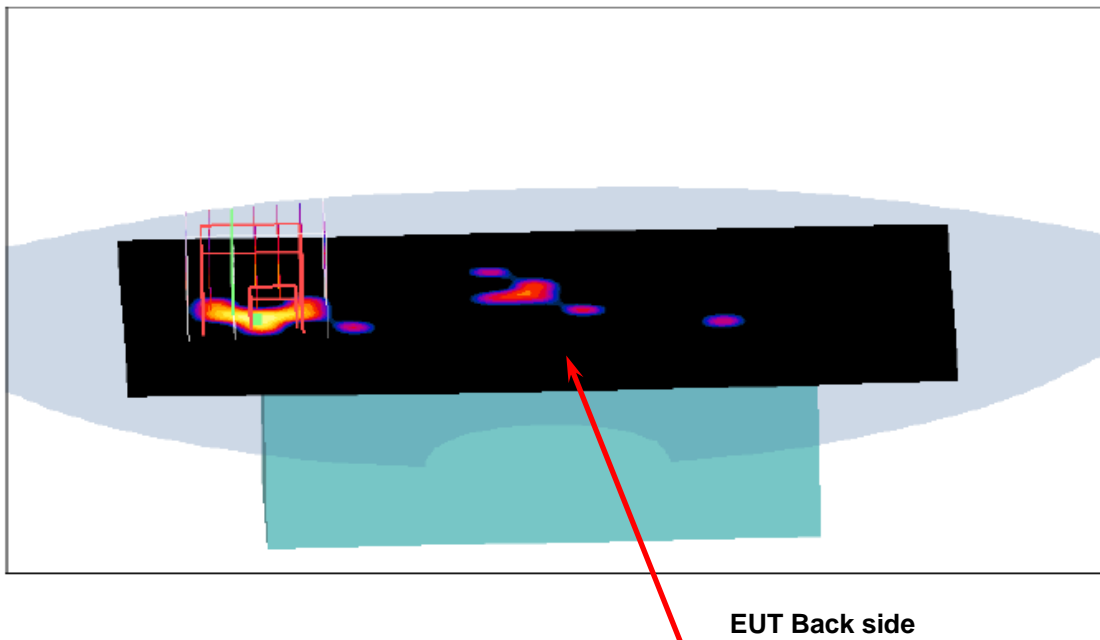
Figure 2. Body SAR Test Setup (Flat Section)
