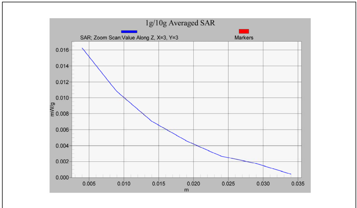
Body SAR Measurement _ CH2 _ close body
