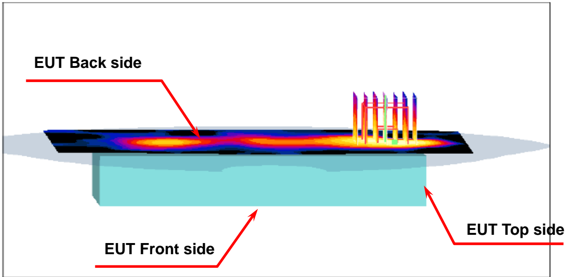
Figure 7. Body SAR Test Setup (Flat Section)
