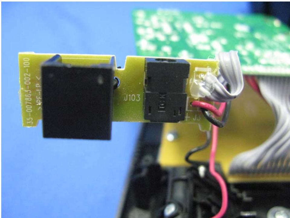
Base Unit AC Jack and Telephone Jack front side
