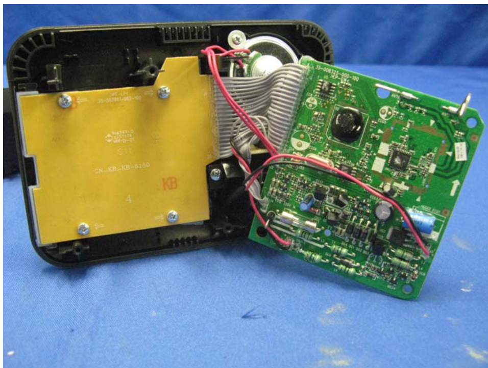
Base Unit assembly (View 2)
