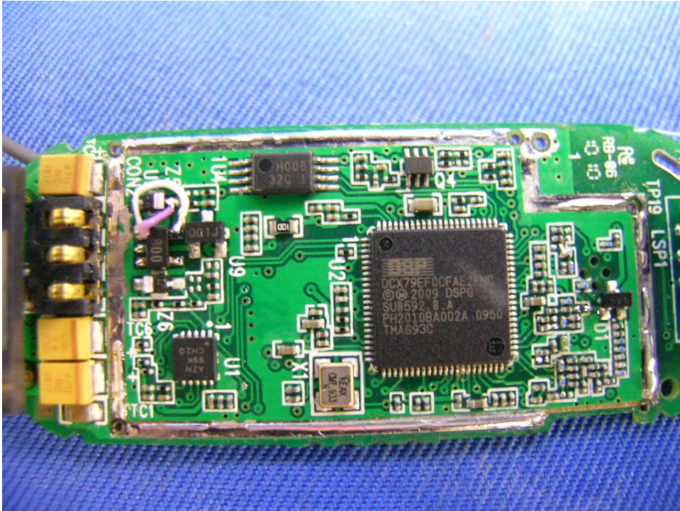
Headset Main PCB comp side (View 3)
