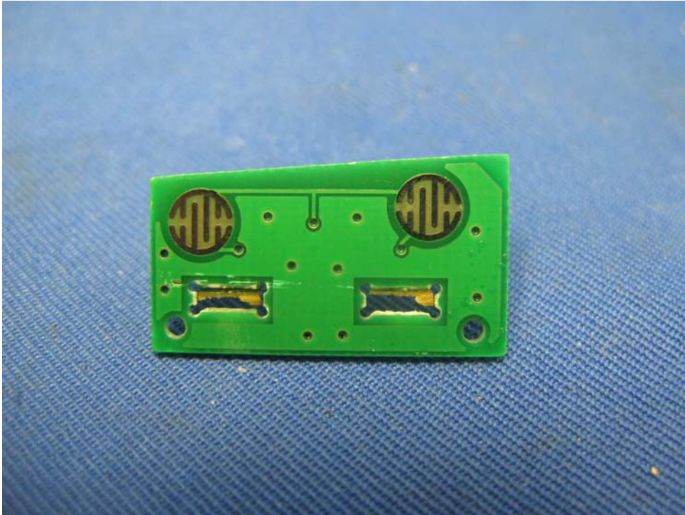
Base Unit Volume Control Key front side
