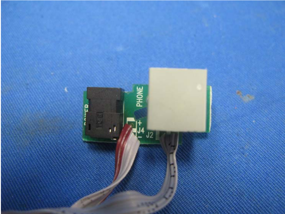
Base Unit Telephone Line Jack front side
