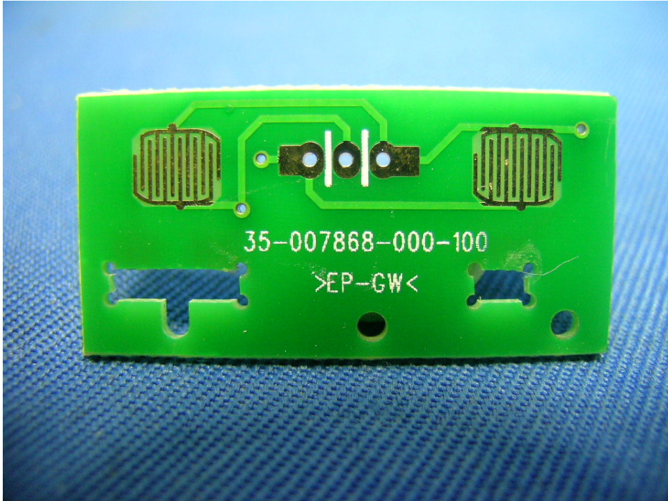
Base Unit Charging Connect rear side
