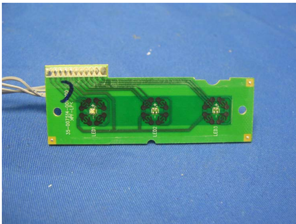
WiFi Gateway LED and Keypad front side
