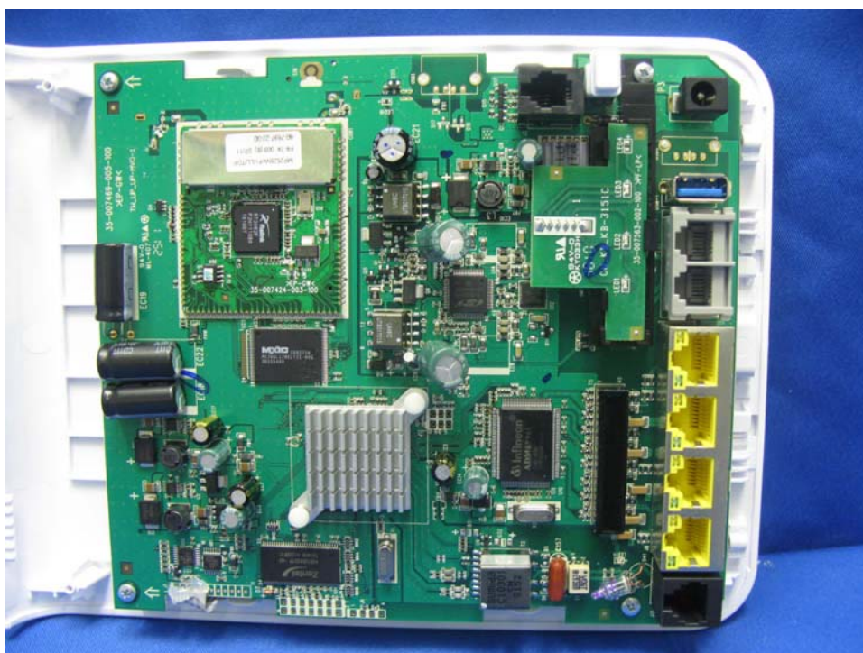
WiFi Gateway Main PCB comp side (View 1)
