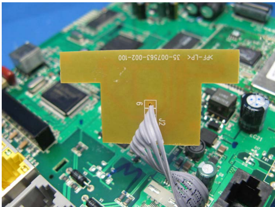
WiFi Gateway LED Board rear side
