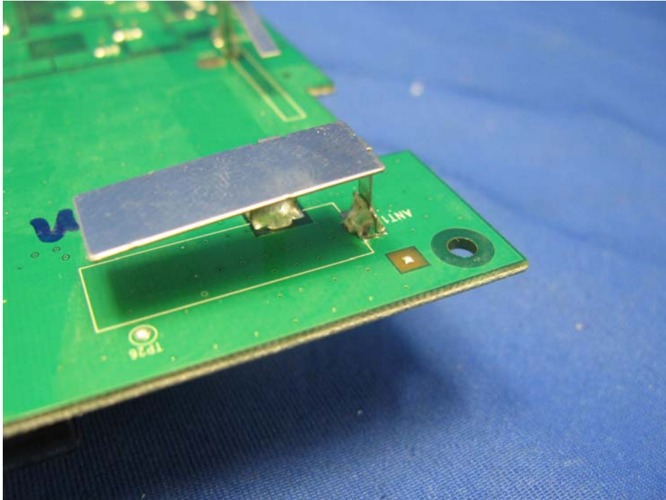
WiFi Gateway Main PCB solder side (View 2)
