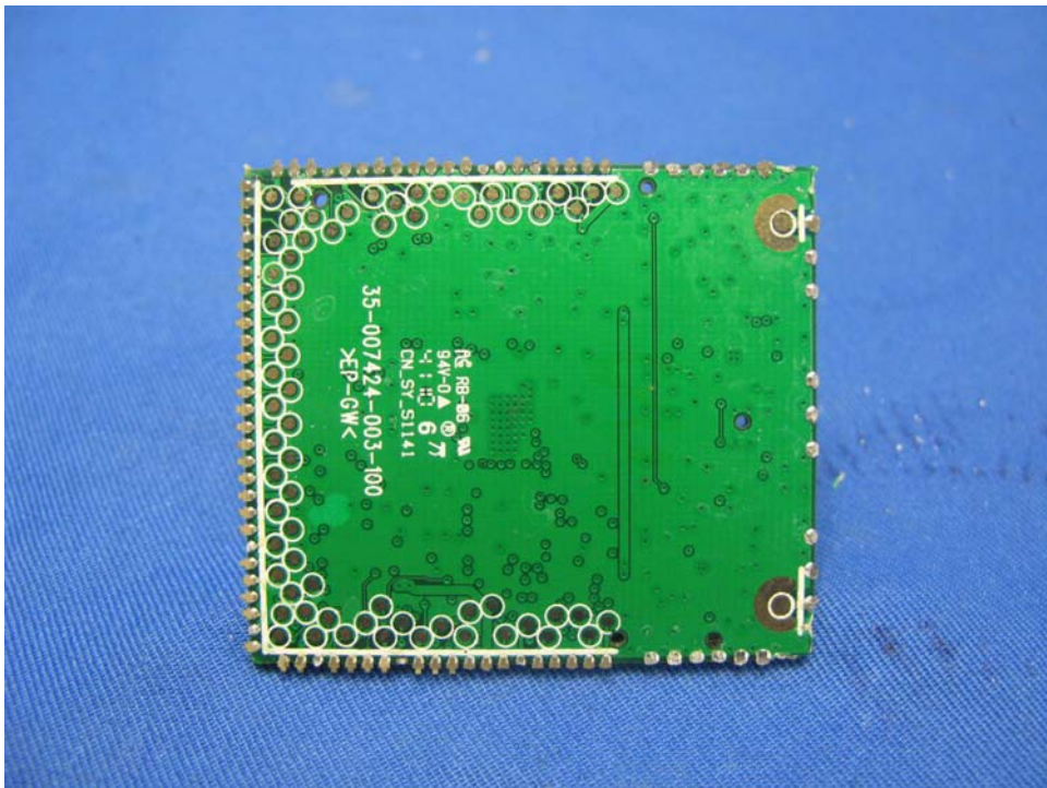
WiFi Gateway WiFi rear side
