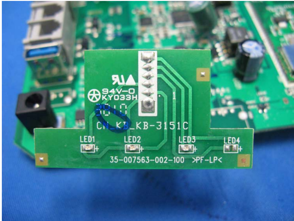
WiFi Gateway LED Board front side
