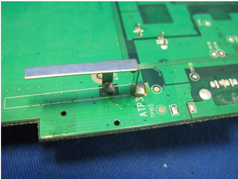
WiFi Gateway Main PCB solder side (View 3)
