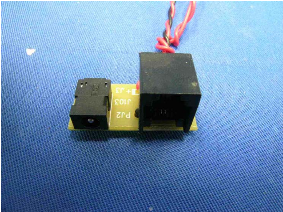
Base Unit Telephone Line Jack and AC Jack front side (View 1)
