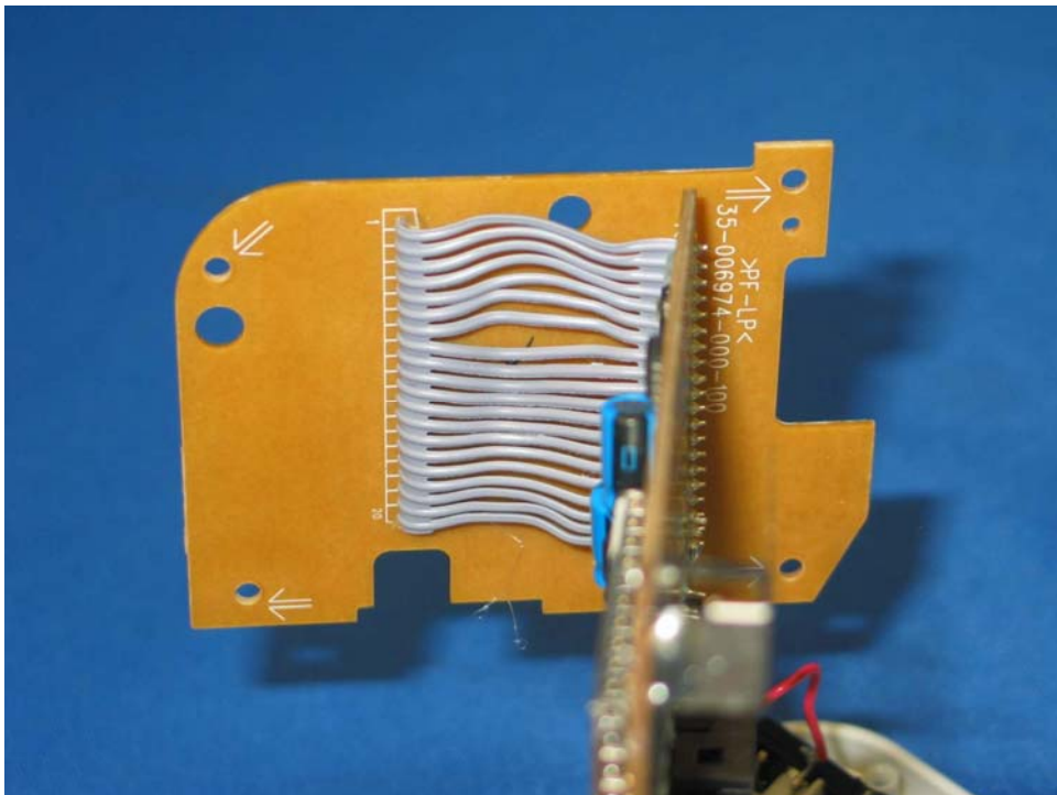
Base Unit DAM rear side (View 2)
