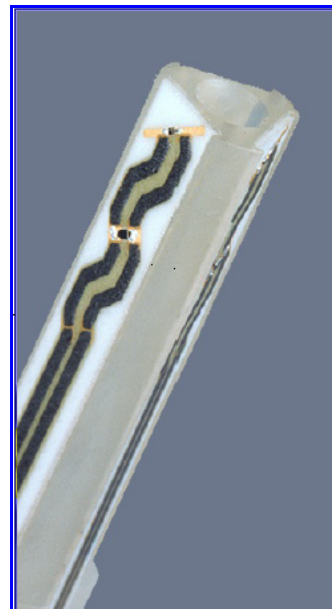
Figure 4. E-field Probe
