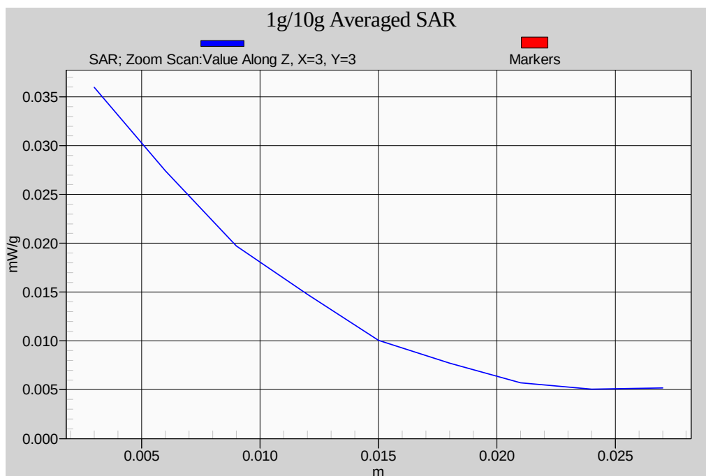
Head SAR Measurement _ Right Cheek CH2
