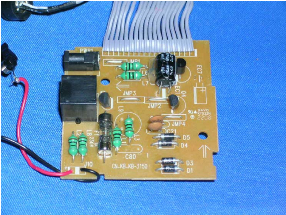
Base Unit Line Interface front side
