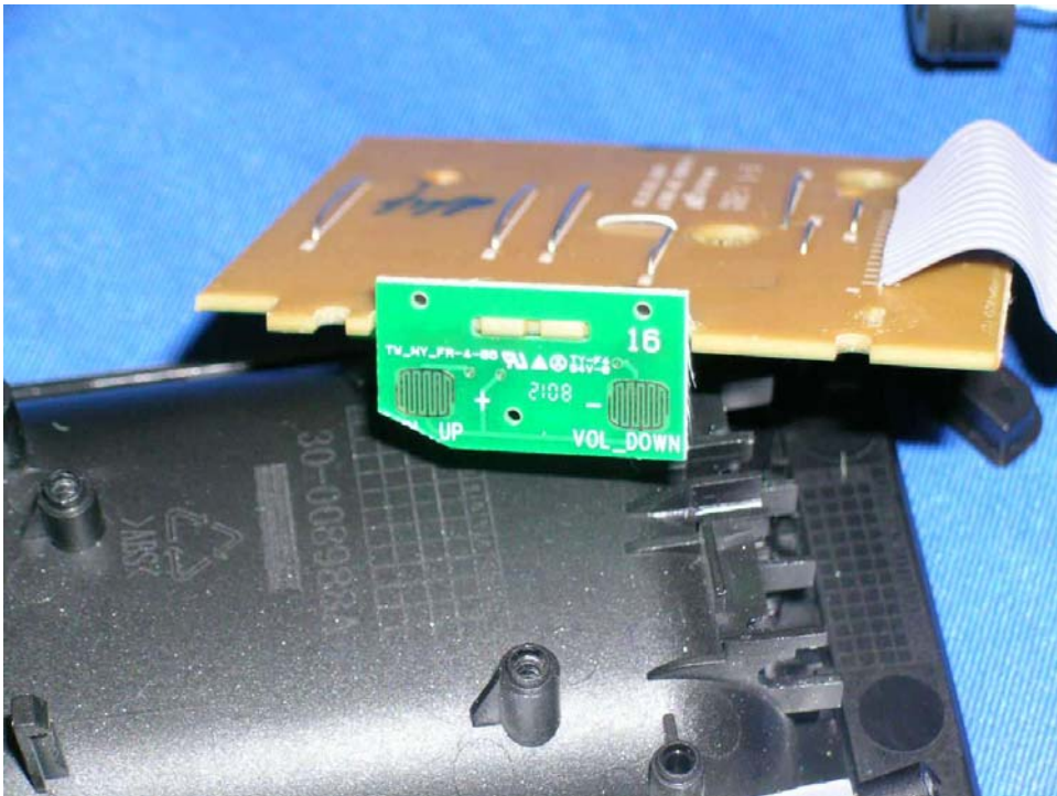
Base Unit DAM front side (View 3)
