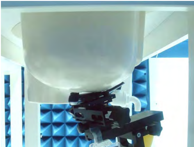
Figure 13. Right Head SAR Test Setup (Cheek)
