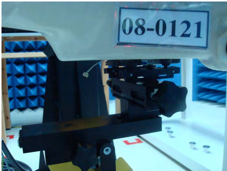
Figure 18. Body SAR Test Setup _ Bottom to Phantom (0mm space)
