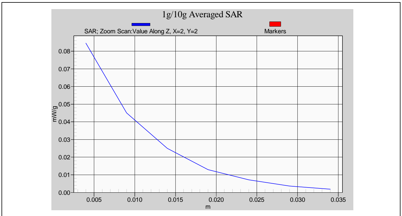
Body SAR Measurement _ CH2
