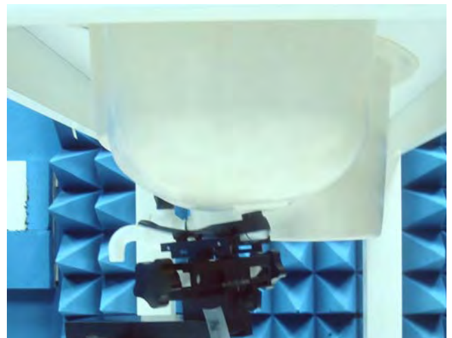
Figure 16. Left Head SAR Test Setup (Tilted)
