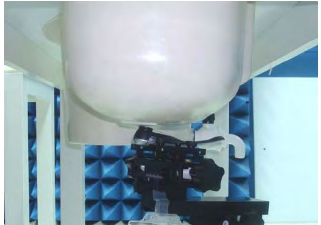
Figure 14. Right Head SAR Test Setup (Tilted)
