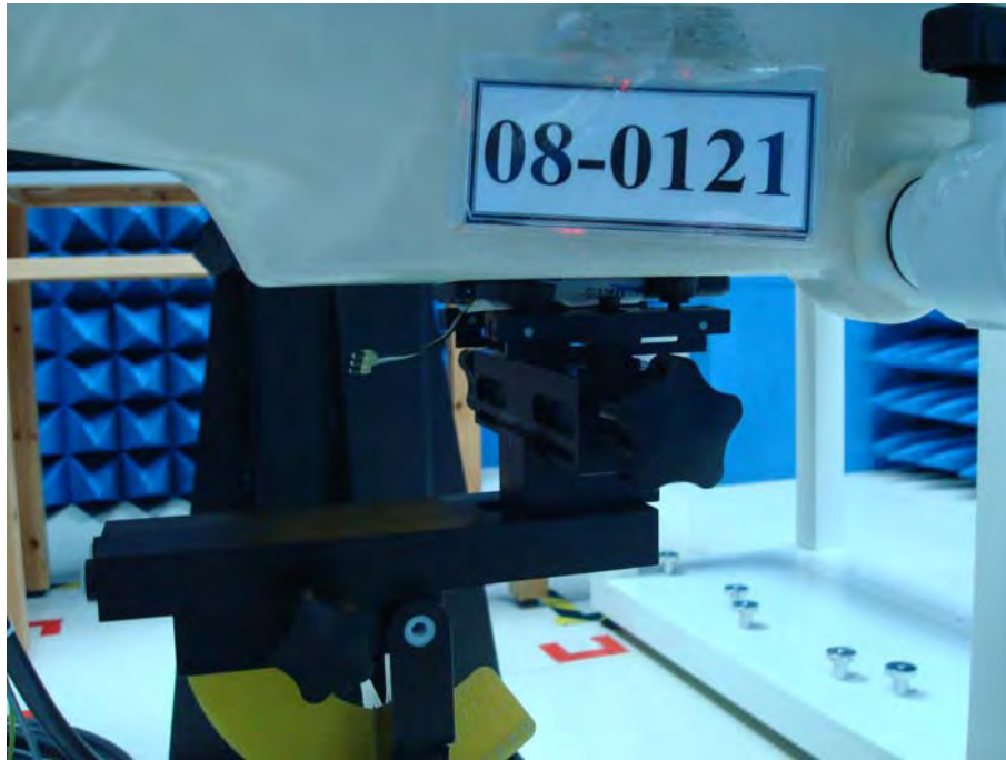
Figure 17. Body SAR Test Setup _ Top to Phantom (0mm space)
