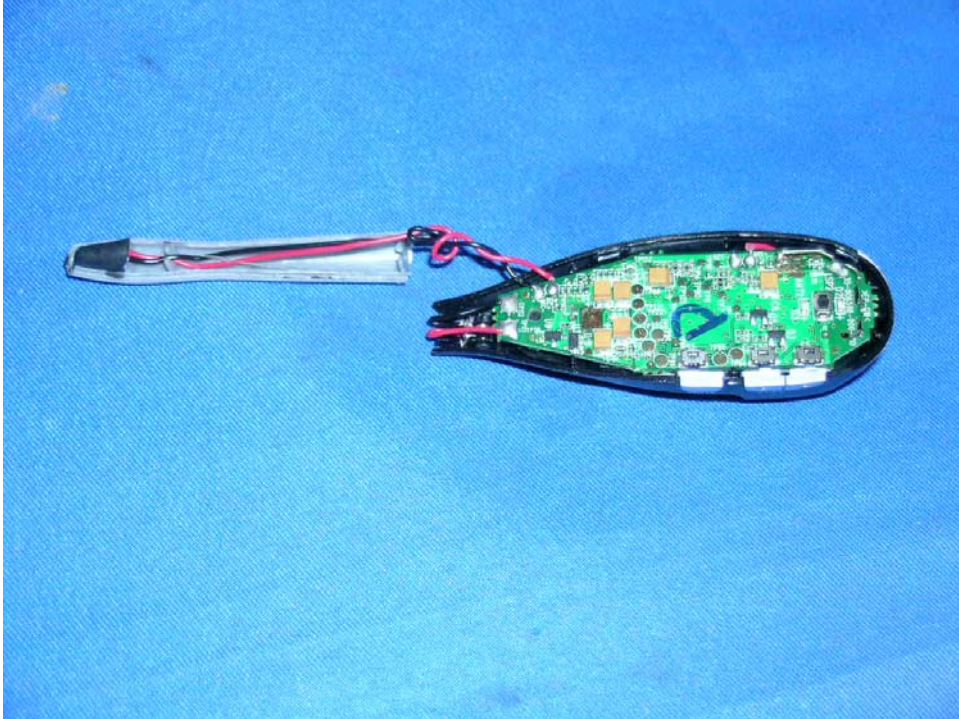
Headset assembly
