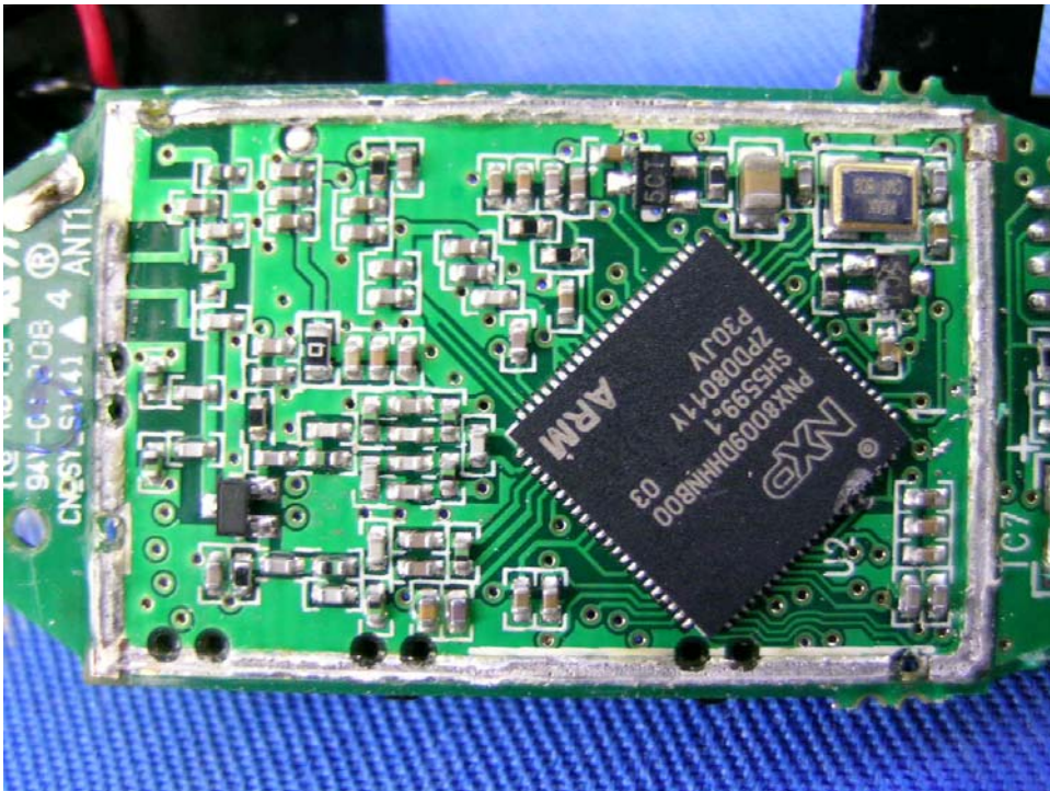
Headset Oscillator PCB comp side
