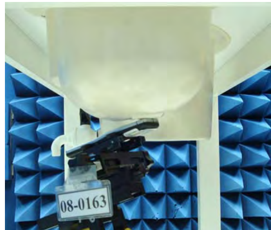
Figure 17. Left Head SAR Test Setup (Tilted)
