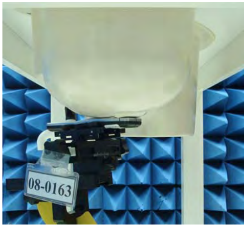
Figure 16. Left Head SAR Test Setup (Cheek)
