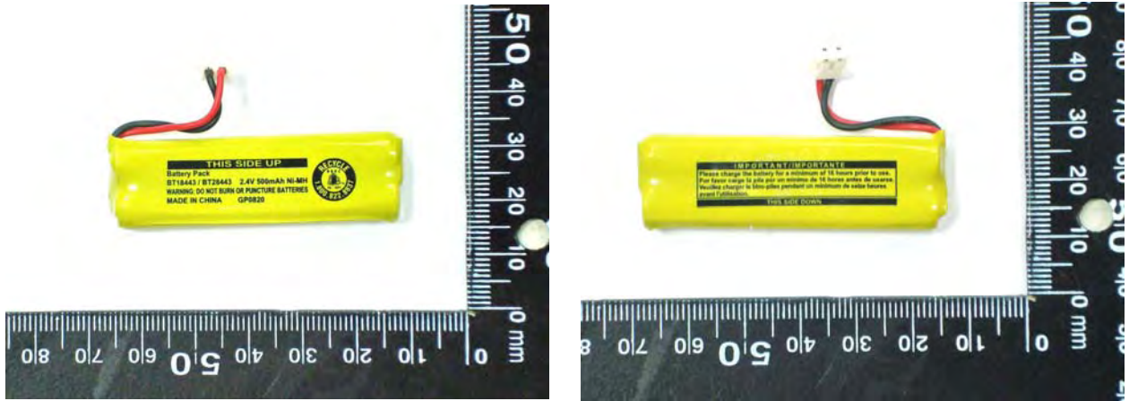
Figure 2. Battery (Ni-MH 2.4V , 500mAh)
