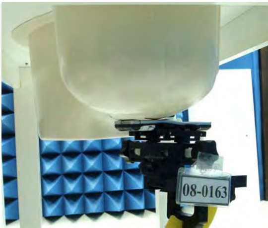
Figure 14. Right Head SAR Test Setup (Cheek)
