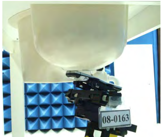
Figure 15. Right Head SAR Test Setup (Tilted)
