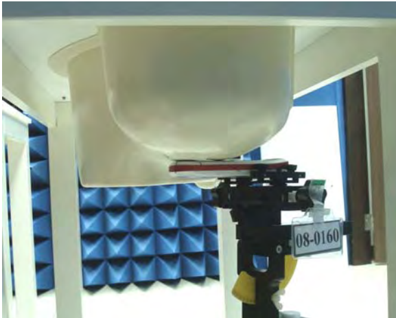
Figure 14. Right Head SAR Test Setup (Cheek)
