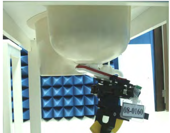
Figure 15. Right Head SAR Test Setup (Tilted)
