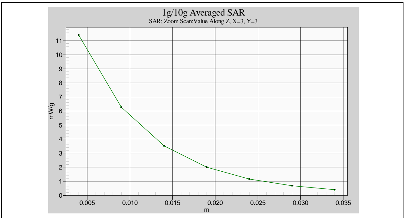
Head -Tissue-Simulating-Liquid 2GHz (2008.03.01)
