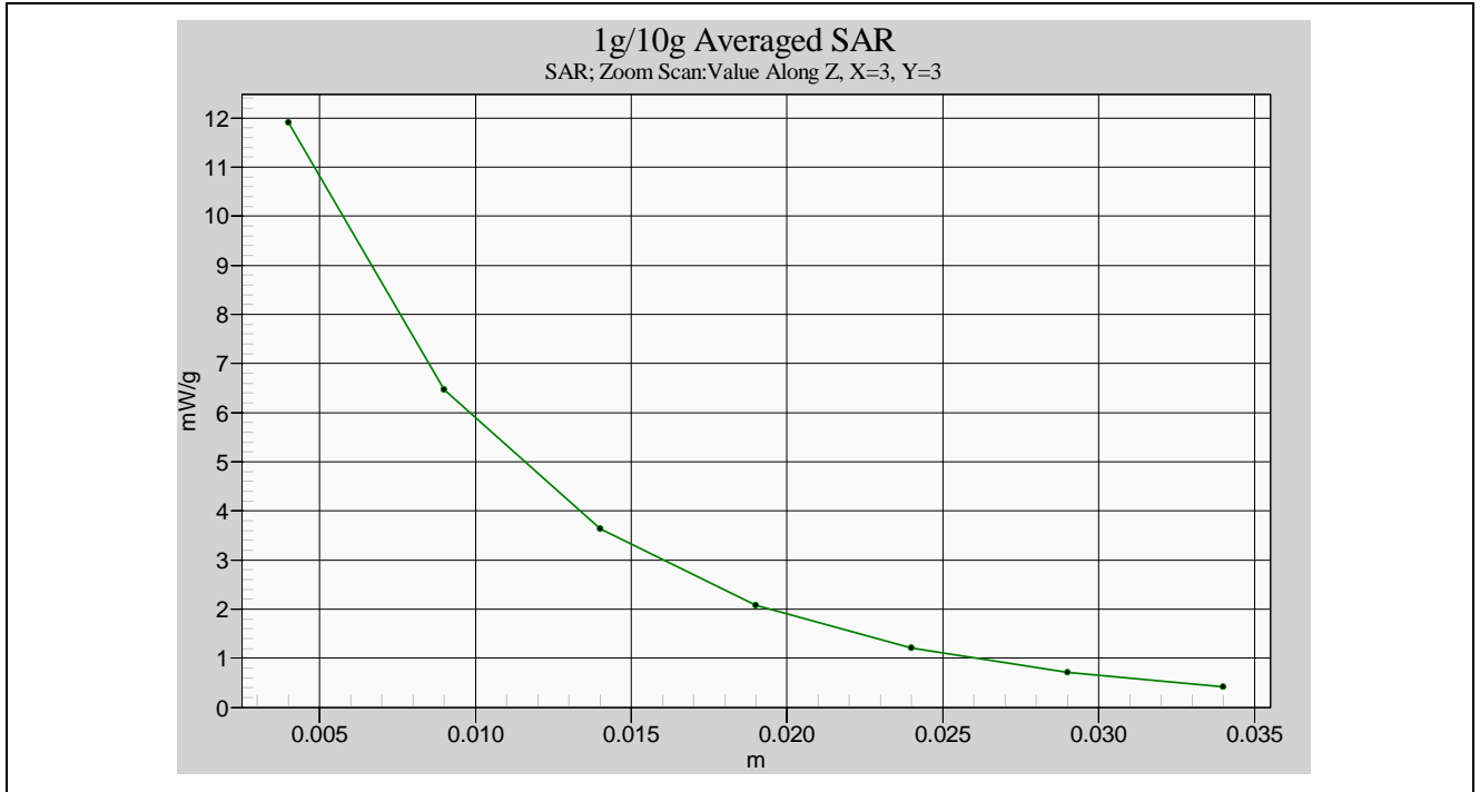
Body -Tissue-Simulating-Liquid 2GHz
