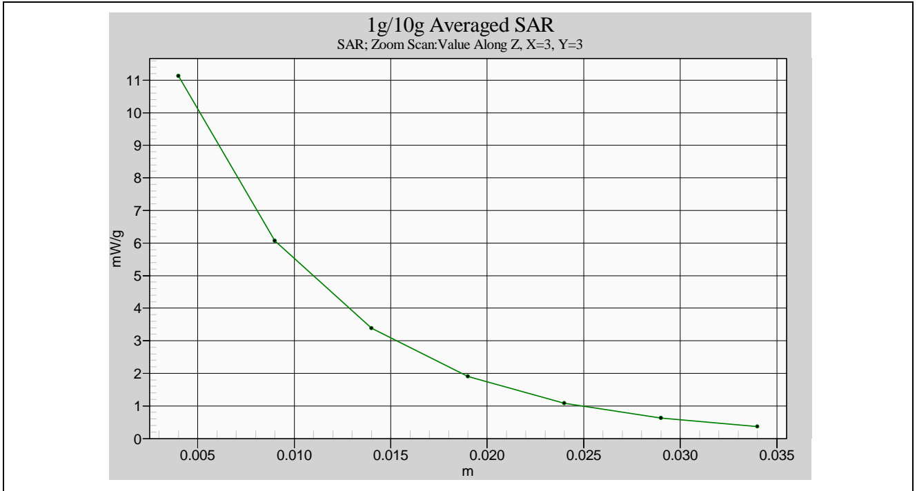
Head-Tissue-Simulating-Liquid 2GHz (2008.0229)
