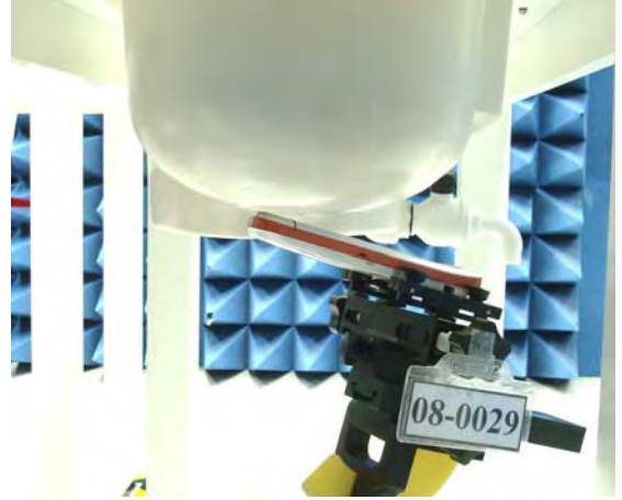
Figure 15. Right Head SAR Test Setup (Tilted)
