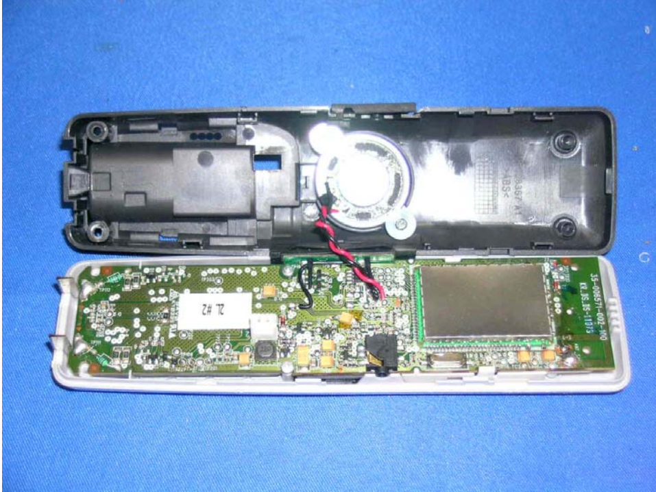
Handset assembly
