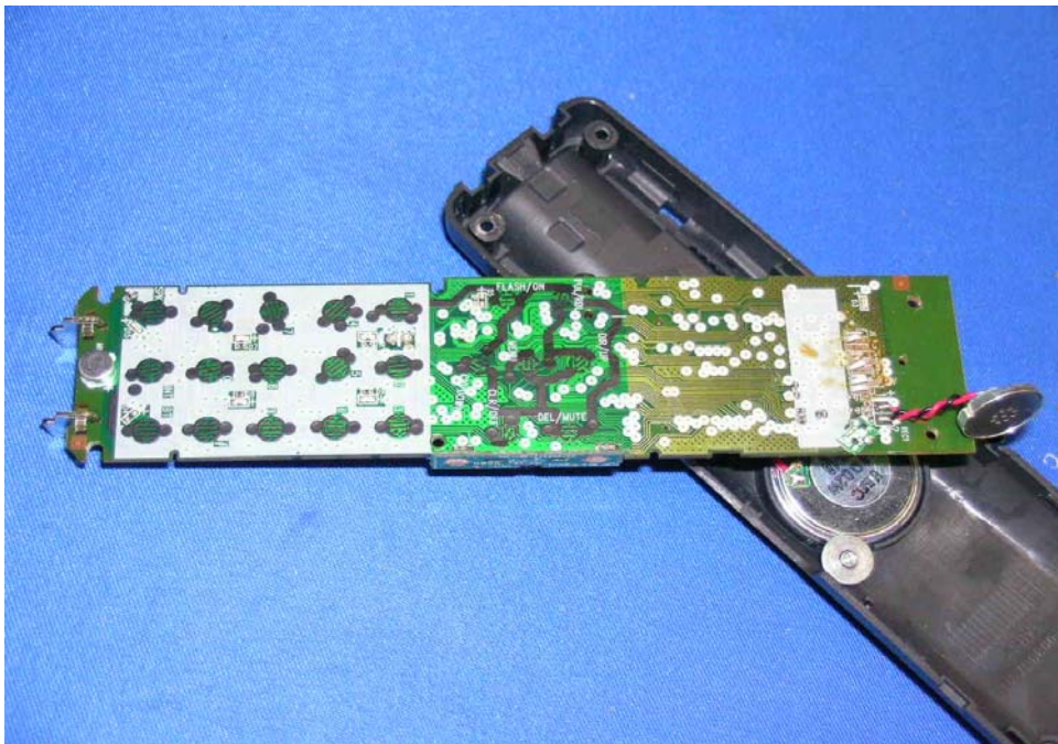
Handset Main PCB display side (View 2)
