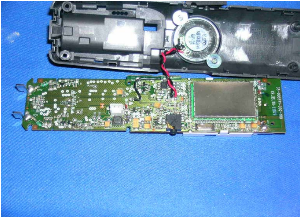
Handset Main PCB comp side
