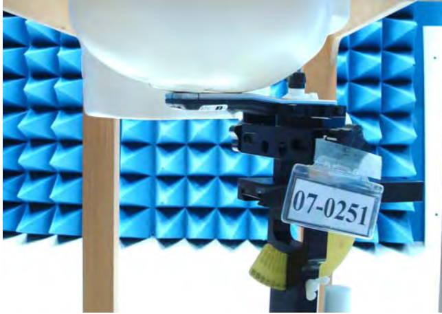
Figure 14. Right Head SAR Test Setup (Cheek)
