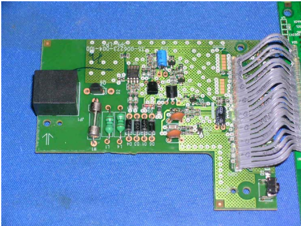
Base Unit another Main PCB comp side (View 1)
