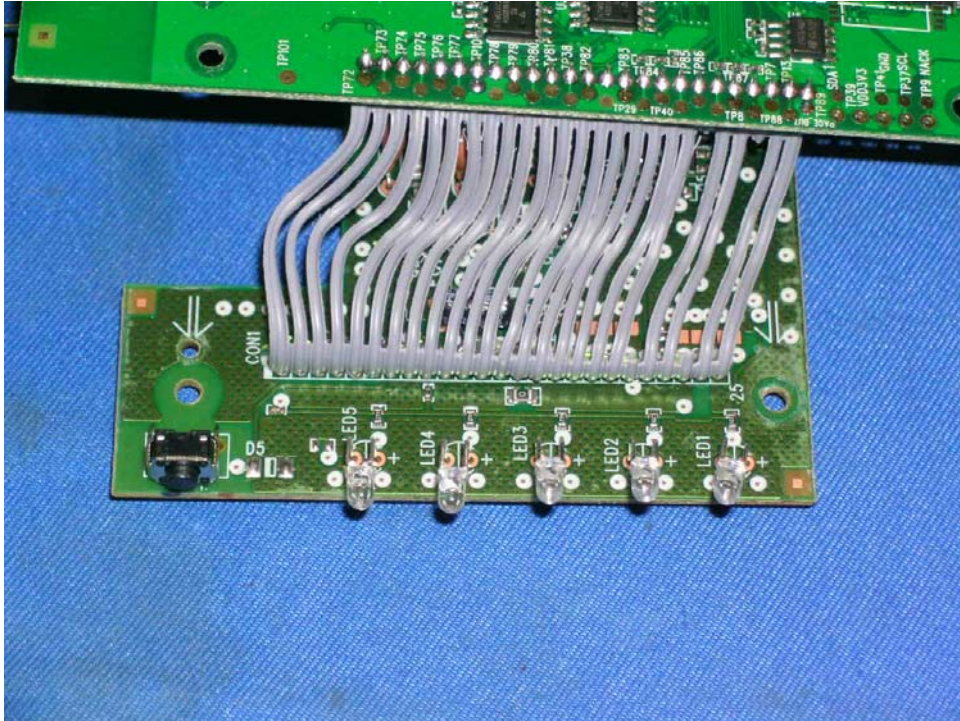
Base Unit another Main PCB comp side (View 2)
