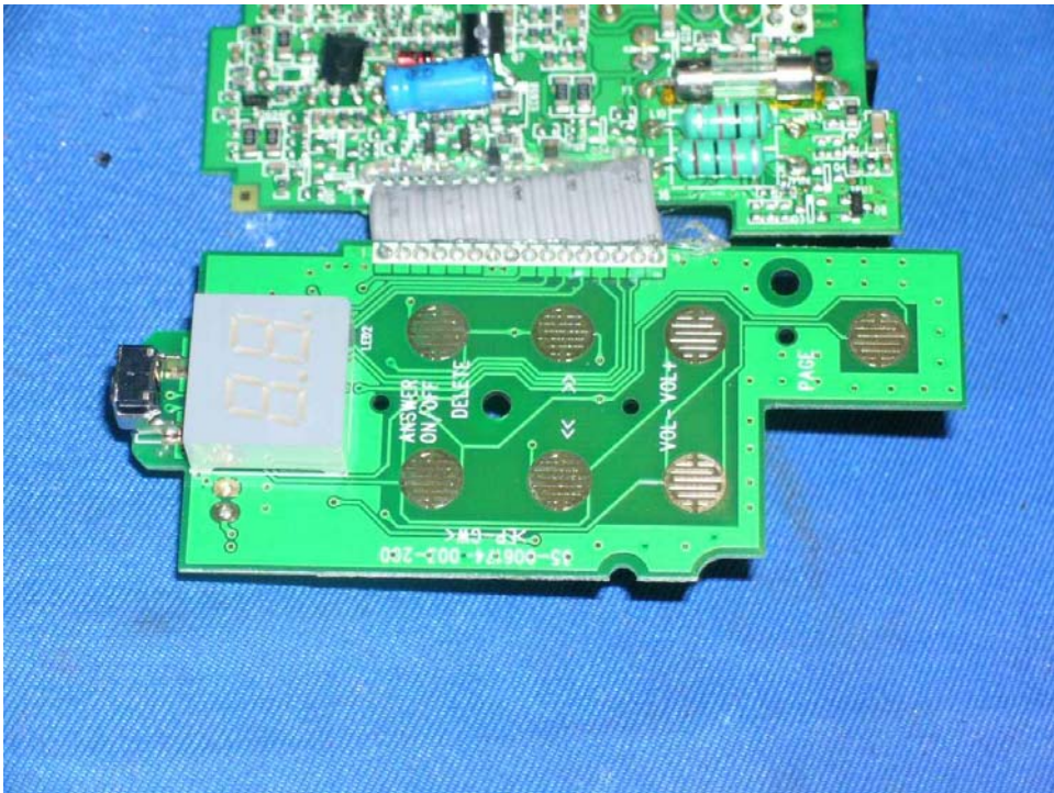
Base Unit Keypad and DAM front side
