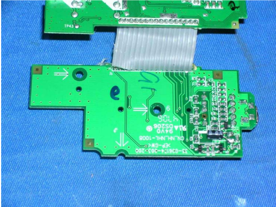
Base Unit Keypad and DAM rear side
