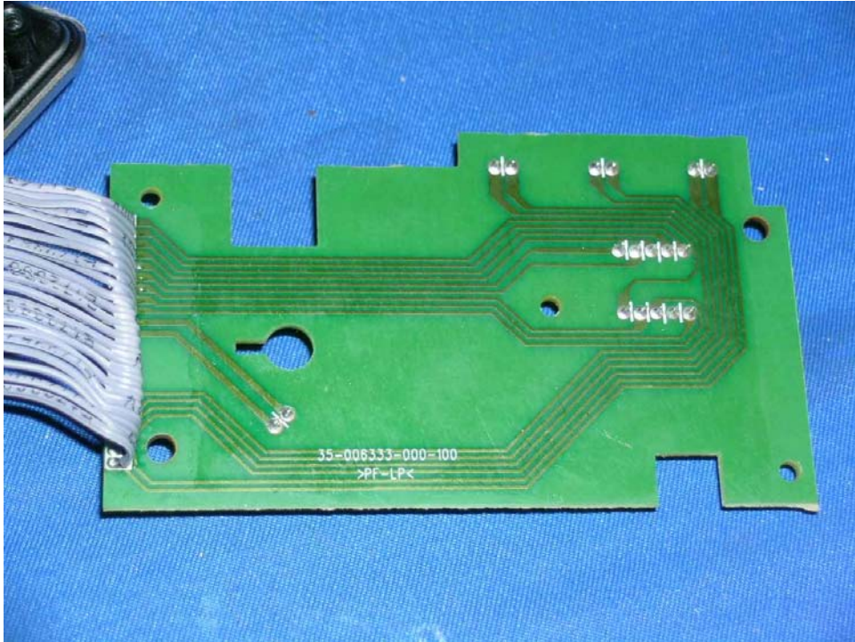
Base Unit Keypad, LED and DAM rear side
