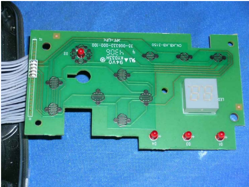
Base Unit Keypad, LED and DAM front side
