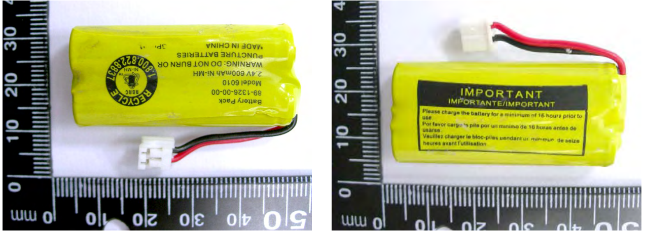
Figure 2. Battery (Ni-MH 2.4V , 600mAh)
