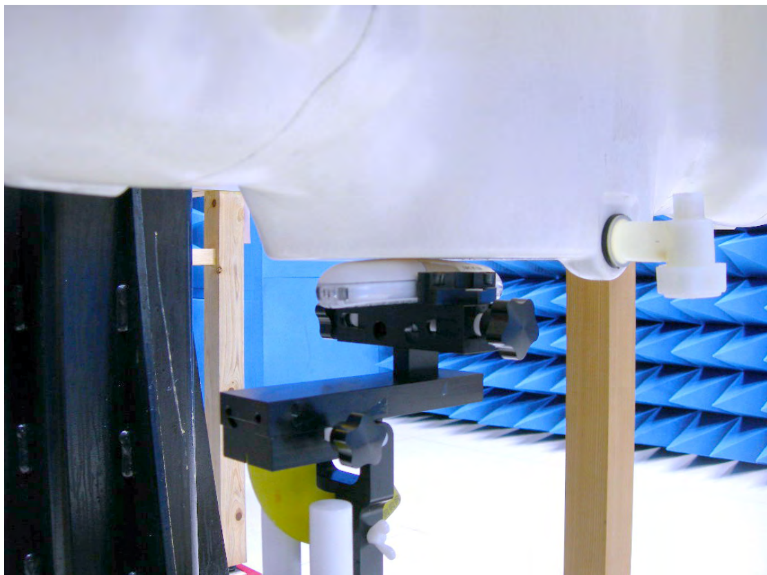
Figure 18. Body SAR Test Setup (Flat Section)
