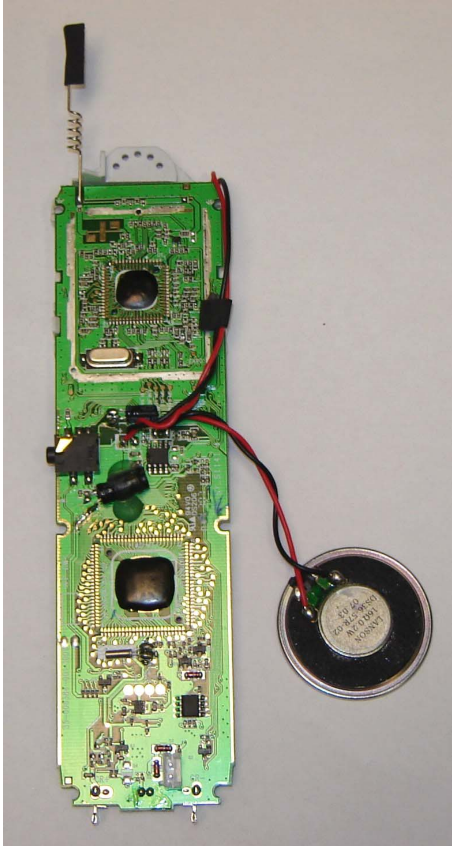
AT&T E5804 - Handset PCB (without shield)
