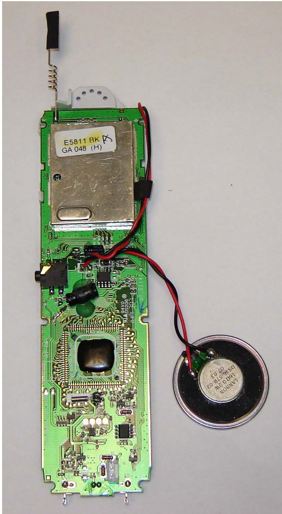
AT&T E5804 - Handset PCB (with shield)
