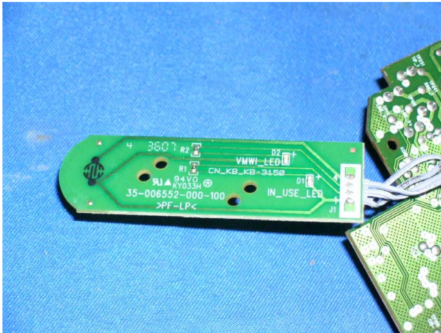
Base Unit LED PCB front side
