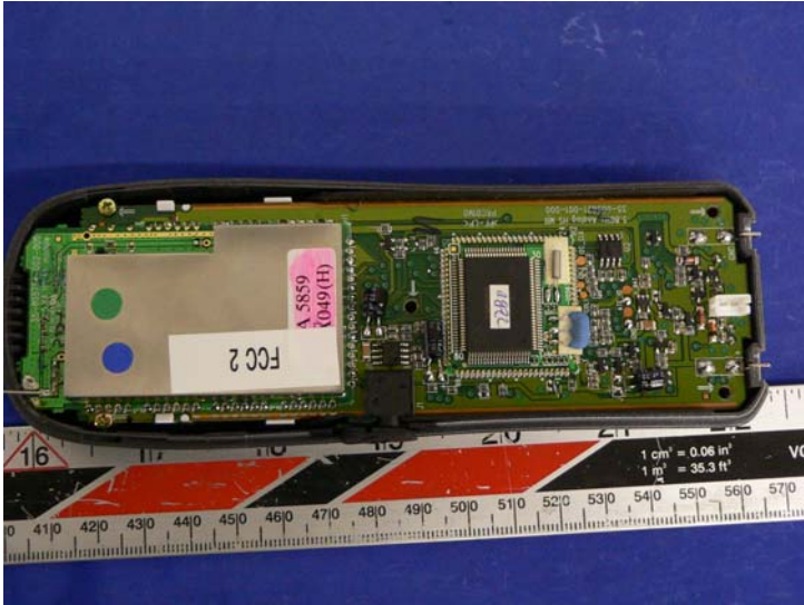
EUT – LC PCB View 1
