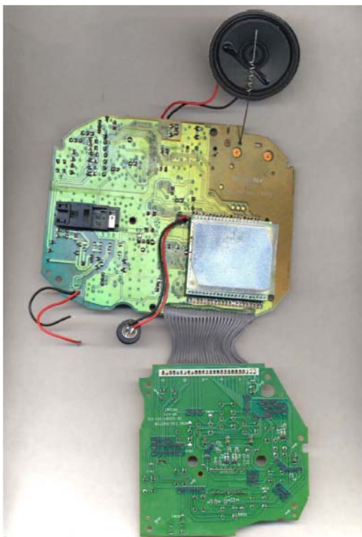
5851 EUT – LC PCB View 3
