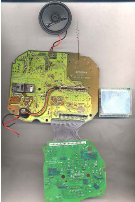
5851 EUT – LC PCB View 5
