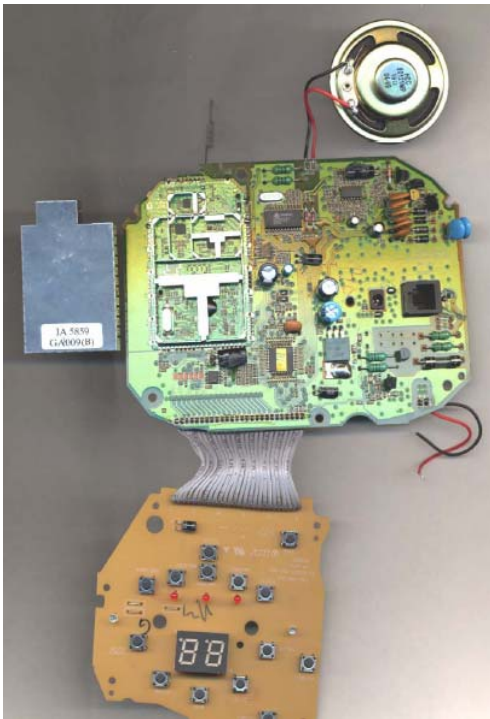
5851 EUT – LC PCB View 3
