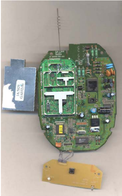
5829 EUT – LC PCB View 3
