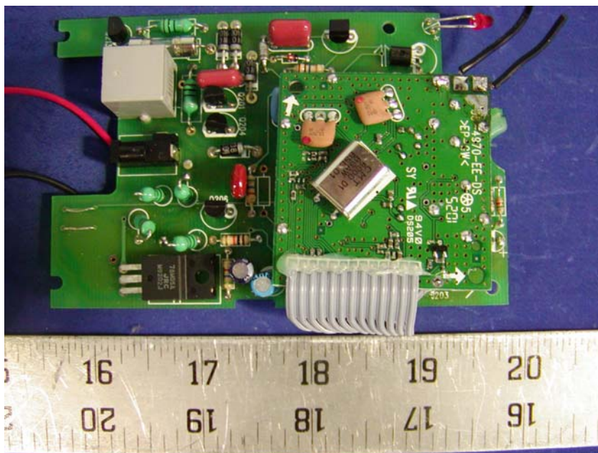
Base - Component View
