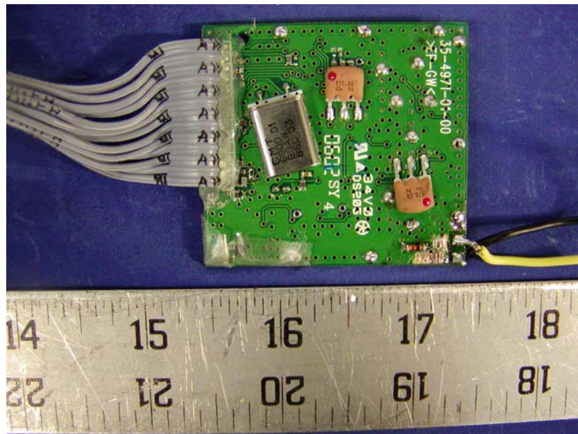
Handset - Transceiver Solder View
