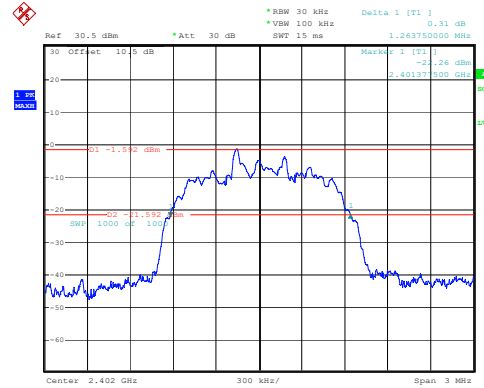
2DH1_Low 1.264MHz
