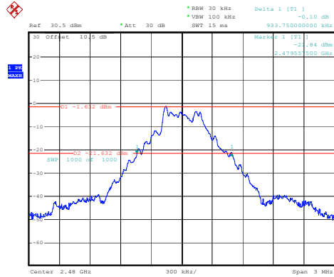
DH1_High 0.934MHz
