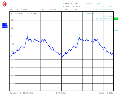
DH1_Low 1.003MHz
