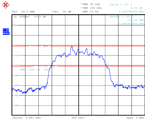
2DH1_Middle 1.264MHz
