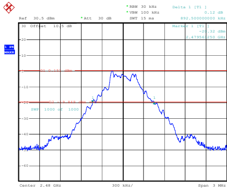
DH1_High 0.893MHz
