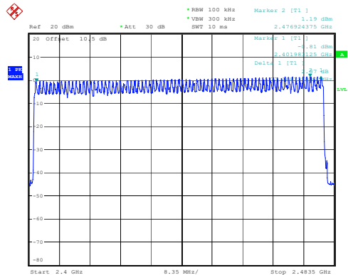
3DH1_Hopping 79
