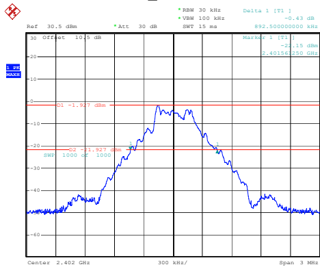
DH1_Low 0.893MHz
