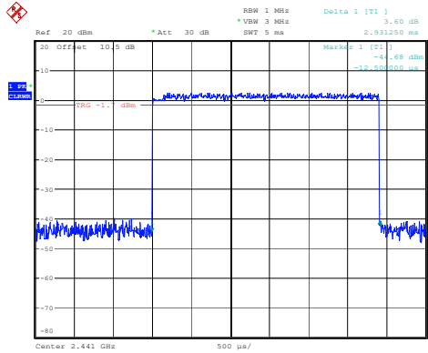
3DH5_Hopping 2.931ms
