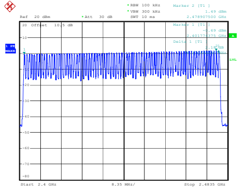
DH1_Hopping 79
