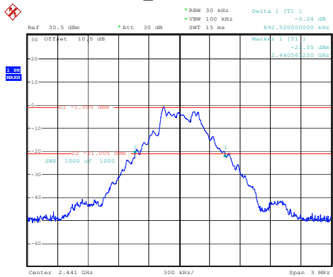
DH1_Middle 0.893MHz
