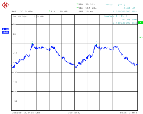
DH1_Middle 1.020MHz
