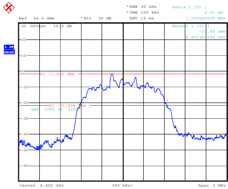
2DH1_Low 1.260MHz
