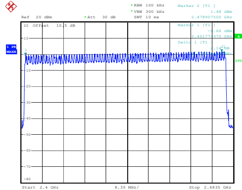
2DH1_Hopping 79
