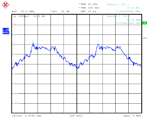
DH1_High 1.003MHz
