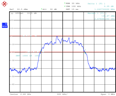
2DH1_High 1.264MHz
