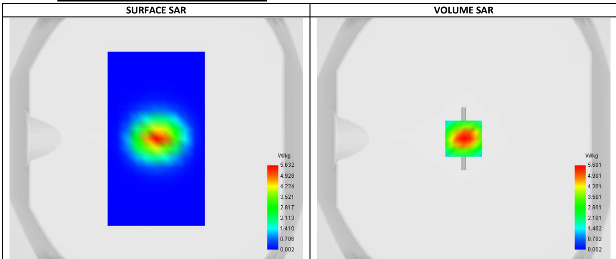
Maximum location: X=0.00, Y=0.00 ; SAR Peak: 9.51 W/kg
