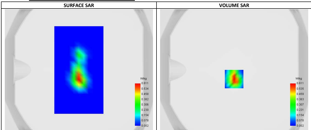
Maximum location: X=0.00, Y=-15.00 ; SAR Peak: 1.24 W/kg
