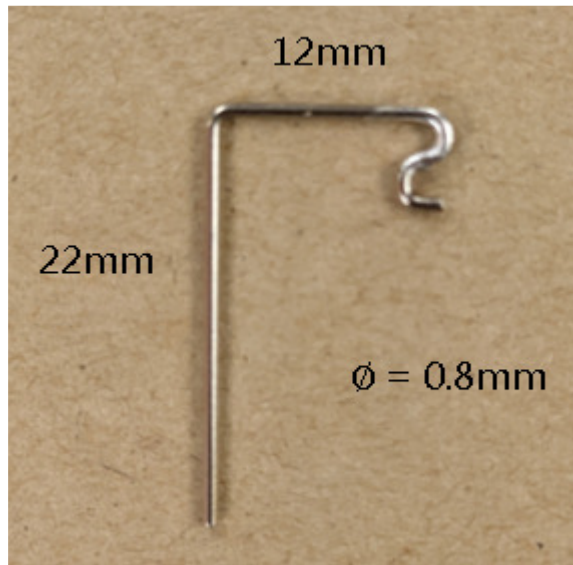
Figure 1 Physical dimension (mm)
