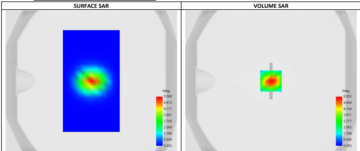
Maximum location: X=0.00, Y=0.00 ; SAR Peak: 9.64 W/kg
