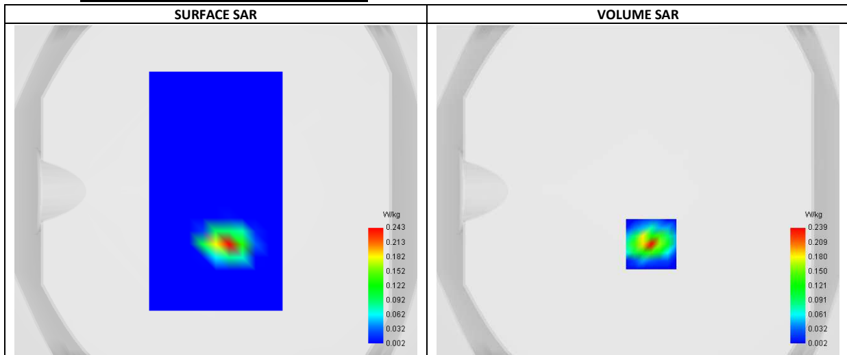
Maximum location: X=8.00, Y=-32.00 ; SAR Peak: 0.60 W/kg
