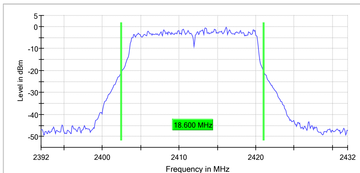
20 dB Bandwidth
