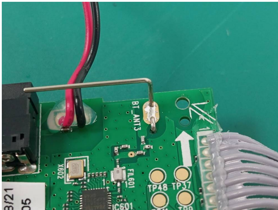
Bluetooth Antenna
