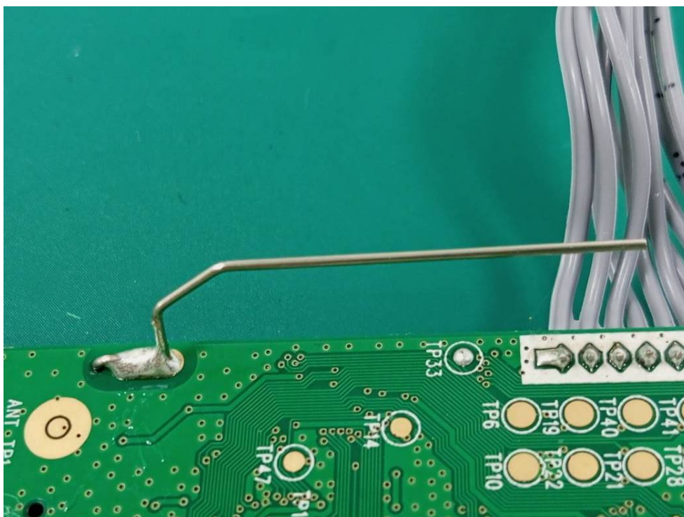
DECT Antenna 1
