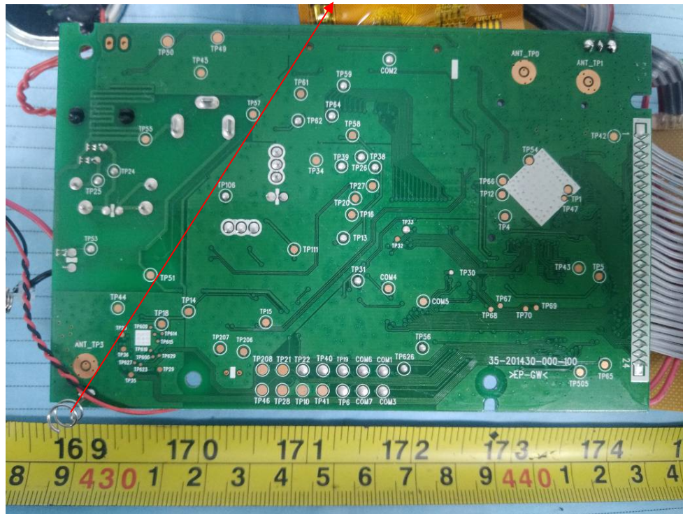
Bluetooth Antenna
