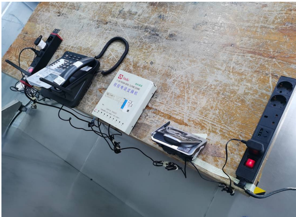
Conducted Emissions Side View adapter 3#
