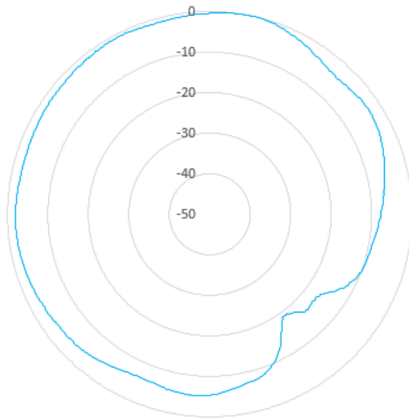
XY Plane (Gain theta)
