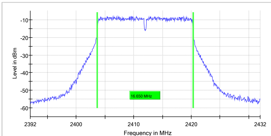
6 dB Bandwidth
