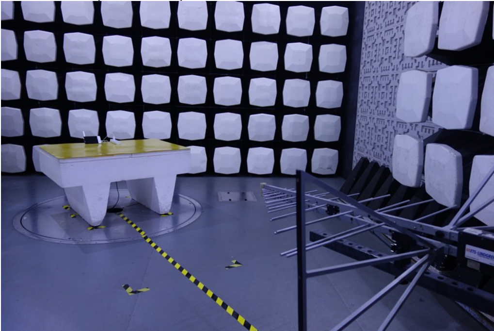
Radiated Emissions (30MHZ-1GHz)
